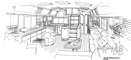
Section A-A Salon looking aft
